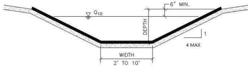
SECTION
