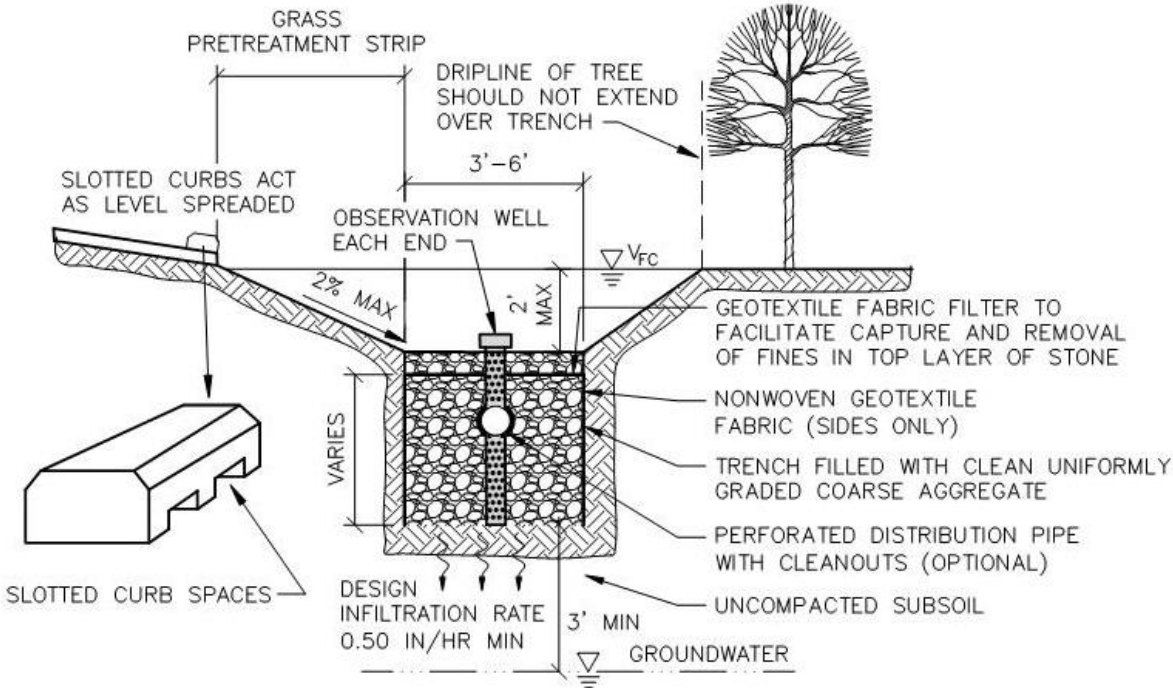
INFILTRATION TRENCH
