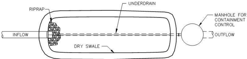
PLAN VIEW
