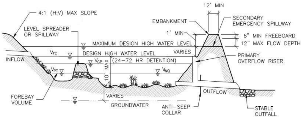
PROFILE
