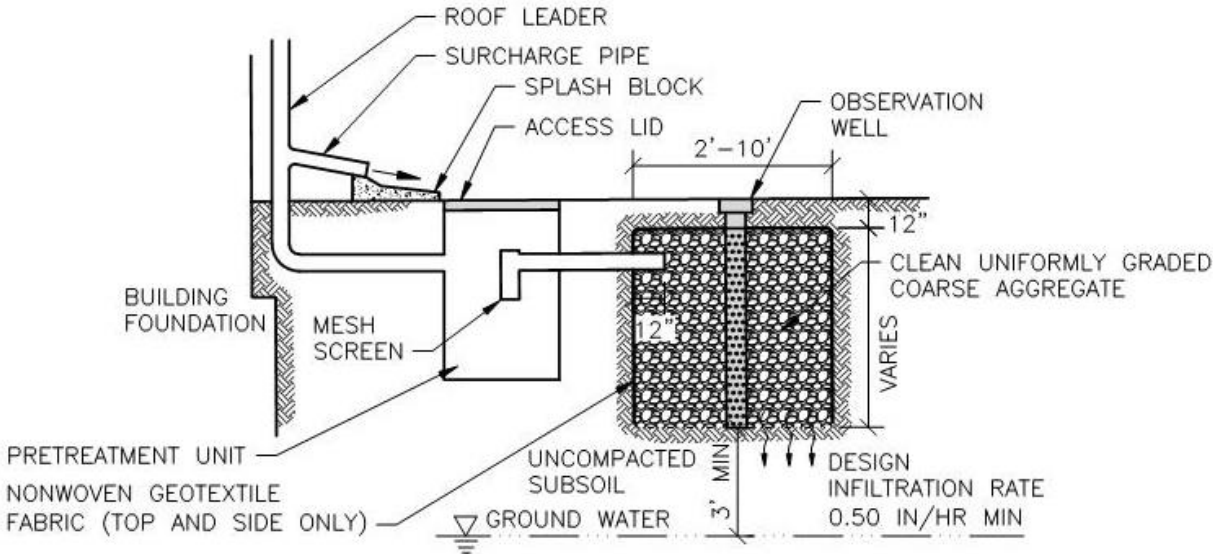
DRY WELL
