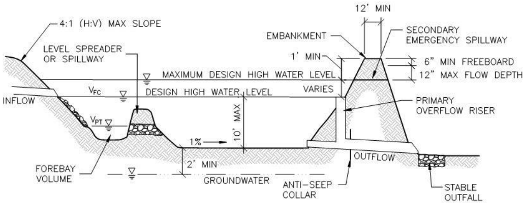
PROFILE
