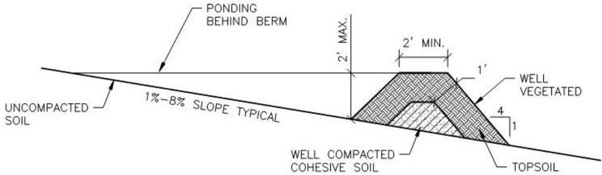
INFILTRATION BERM
