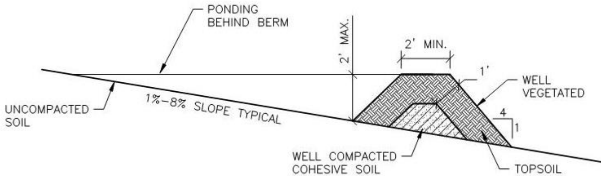
INFILTRATION BERM
