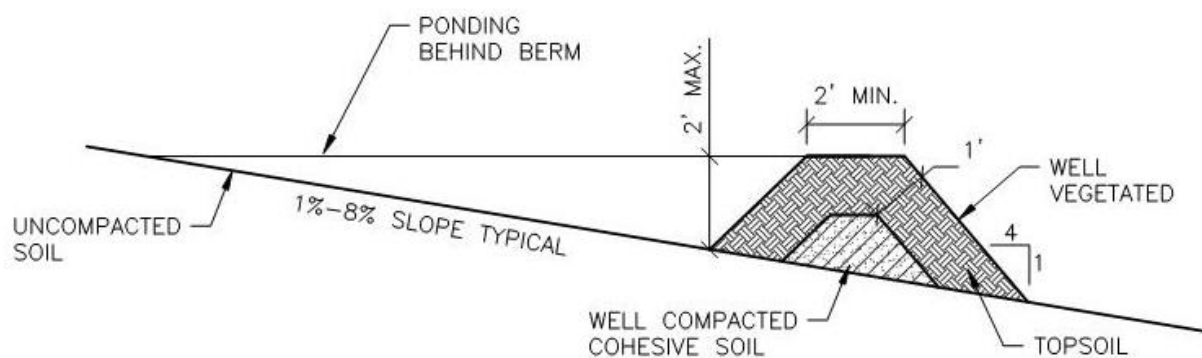
INFILTRATION BERM
