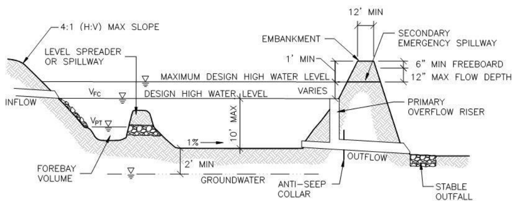
PROFILE
