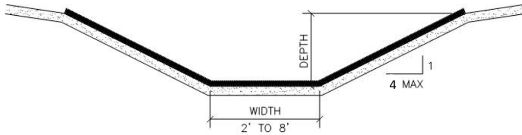
SECTION
