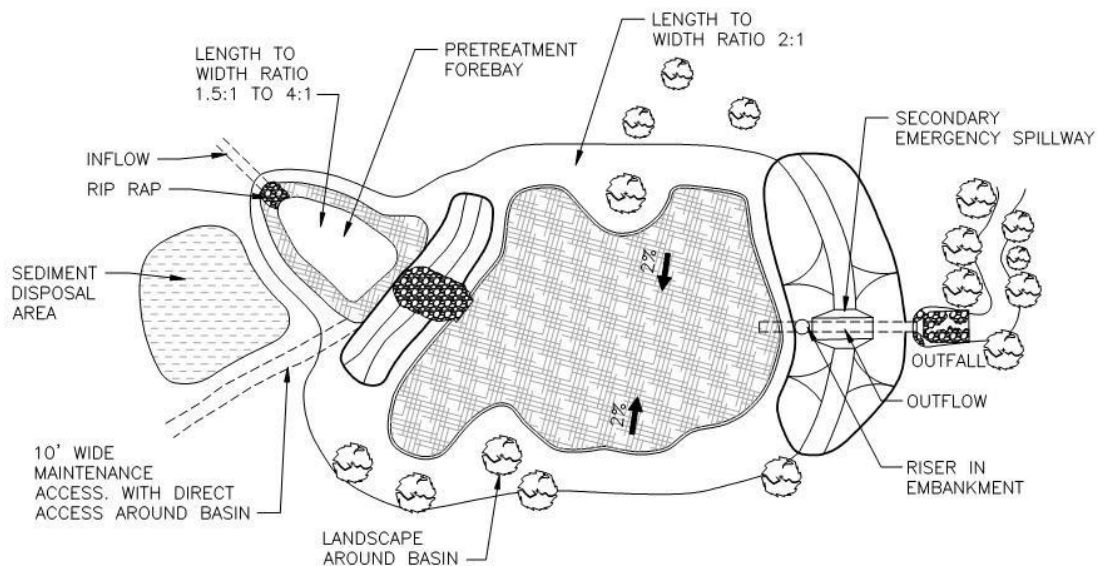
PLAN VIEW
