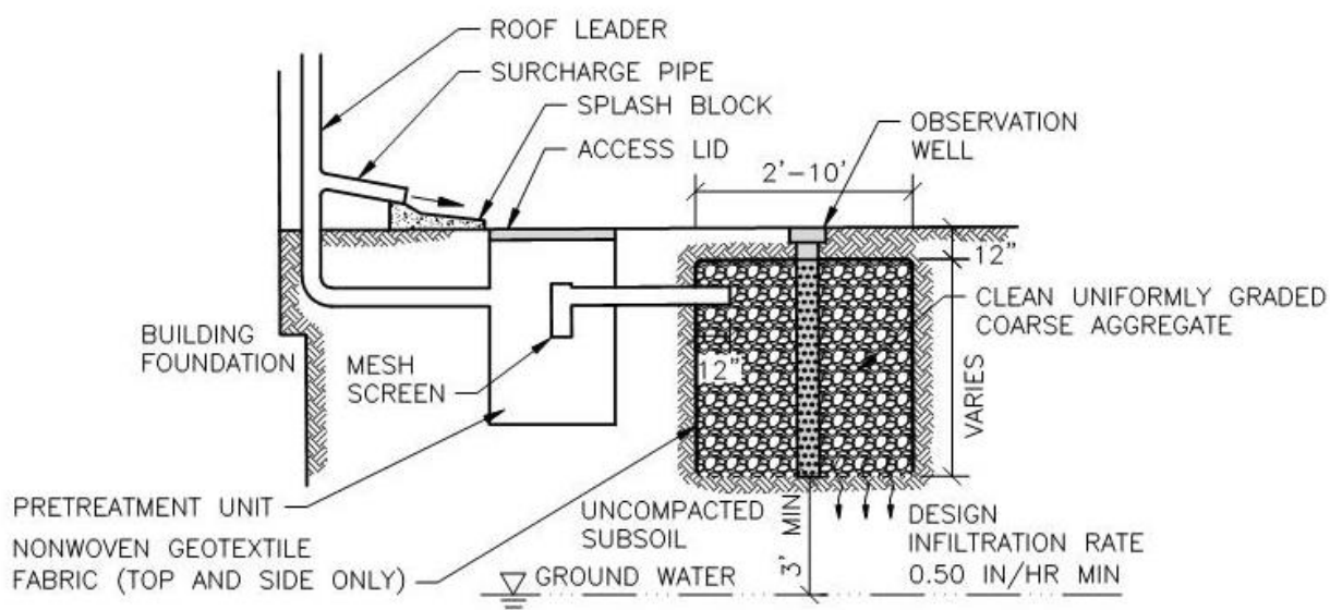
DRY WELL
